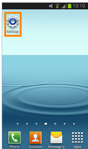
Settings
