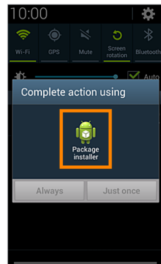
Package installer
