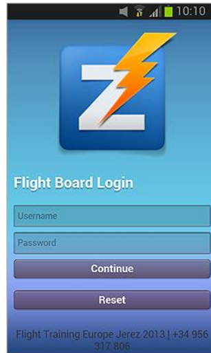
Login screen
