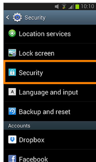
Security
